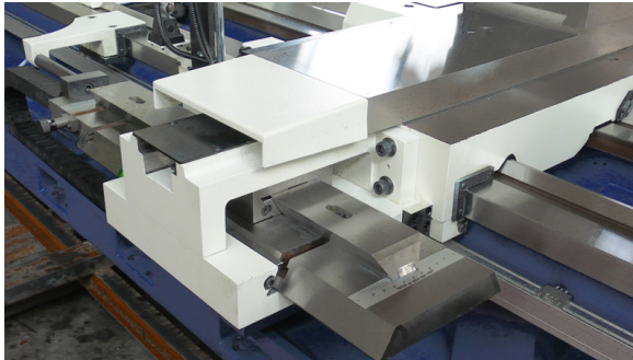
Roller-tipped steady rest
